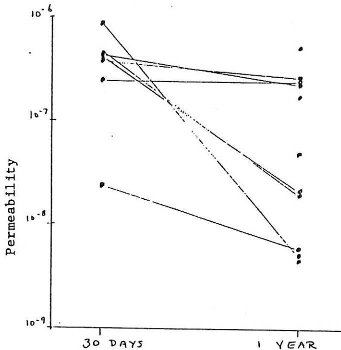
Figure 7. Permeability of Mixed Samples Vs. Time Shallow Soil Mixing Case Study
