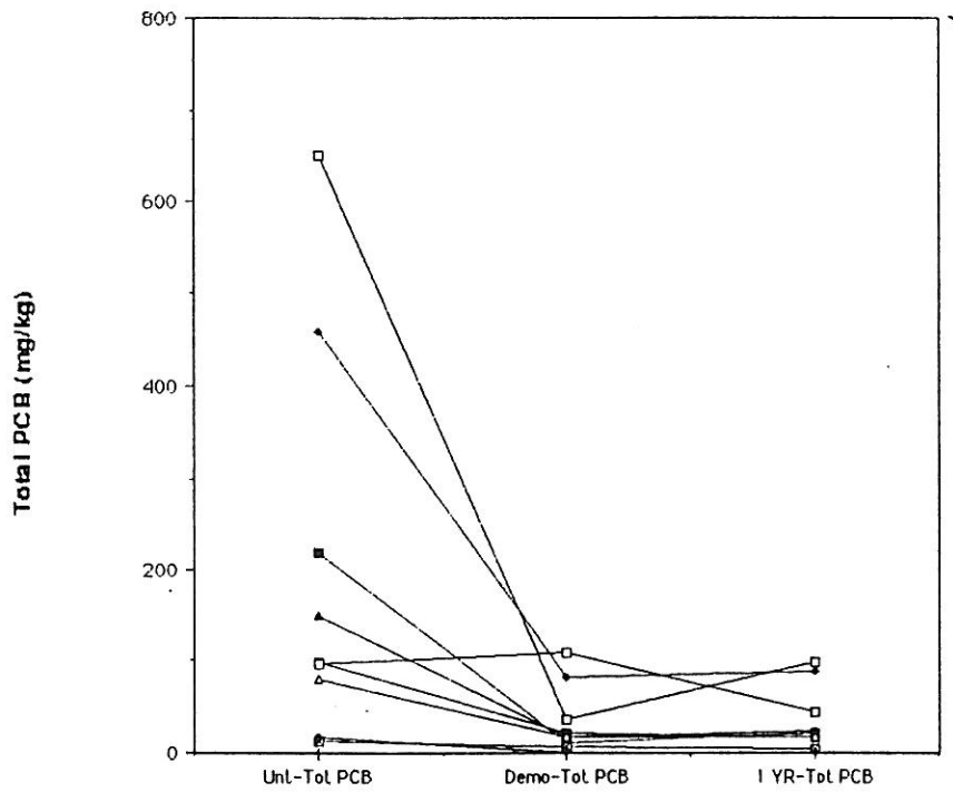
Figure 5. PCB Concentration Before and After Treatment
