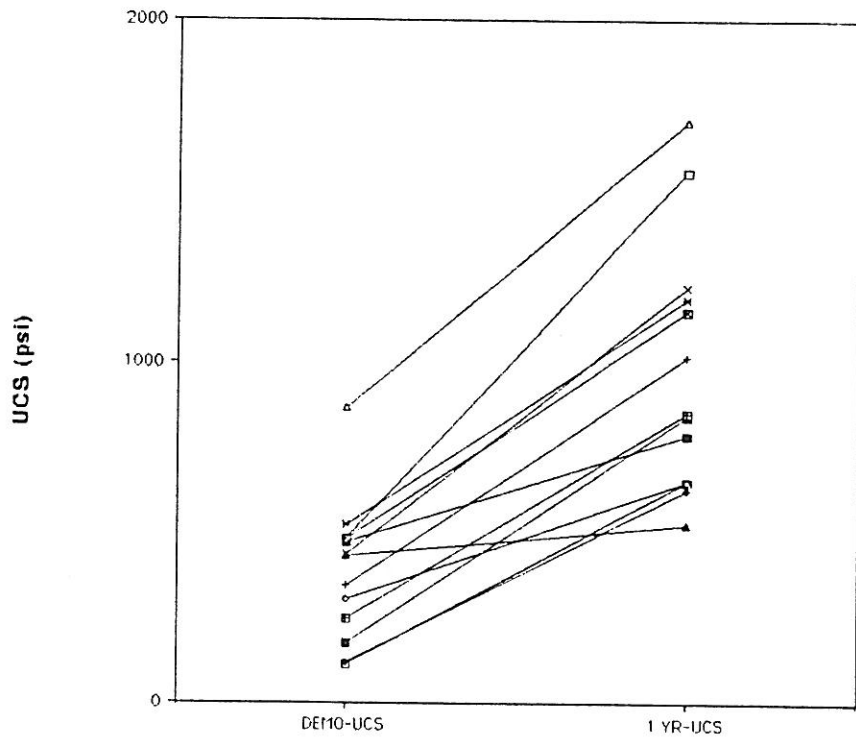
Figure 6. Unconfined Strength of Mixed Samples Vs. Time
